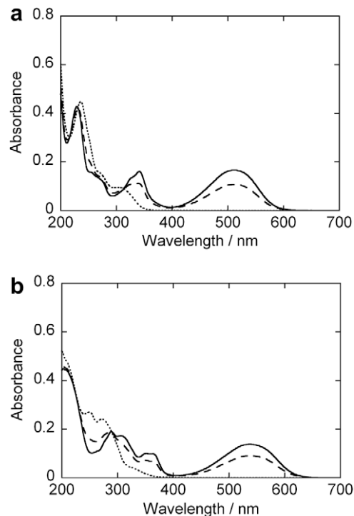
Figure 1. Absorption spectra of 1 (a, 1.90 \times 10^{-5} M) and 2 (b, 1.32 \times 10^{-5} M) in hexane. Dotted lines: open-ring isomers 1a and 2a , solid lines: closed-ring isomers 1b and 2b , dashed lines: photostationary states under irradiation with 300 nm light.
