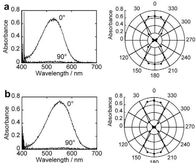
Figure 3. Polarized absorption spectra and polar plots of the absorbance for UV-irradiated single-component crystals of 1a (a) and 2a (b).
